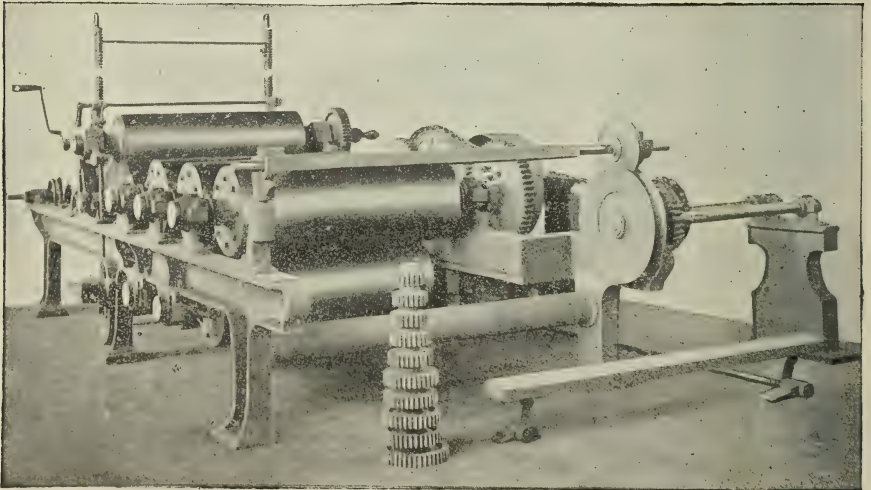
FIG. 121.—Asphalt Saturator.
